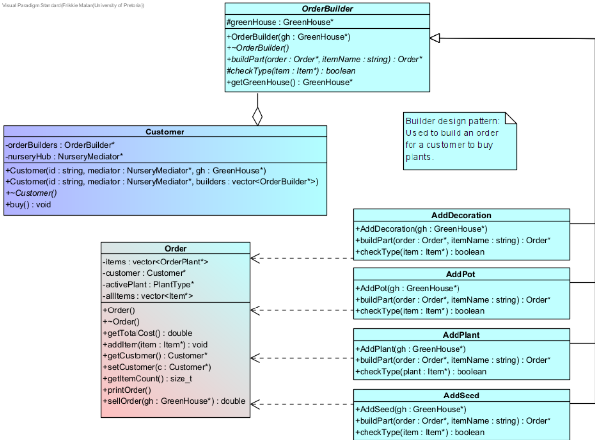
Figure 3. Builder patten.
